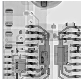
Semiconductor inspection
