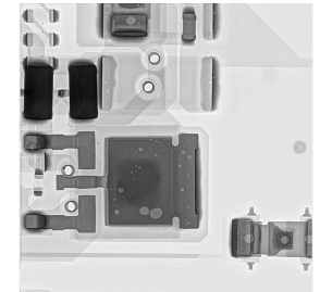
IGBT
