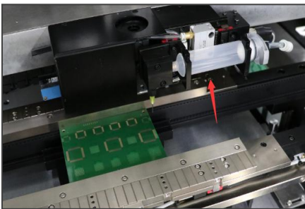
Auto Glue Dispensing
